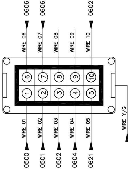
CONN. 10P FEMALE
