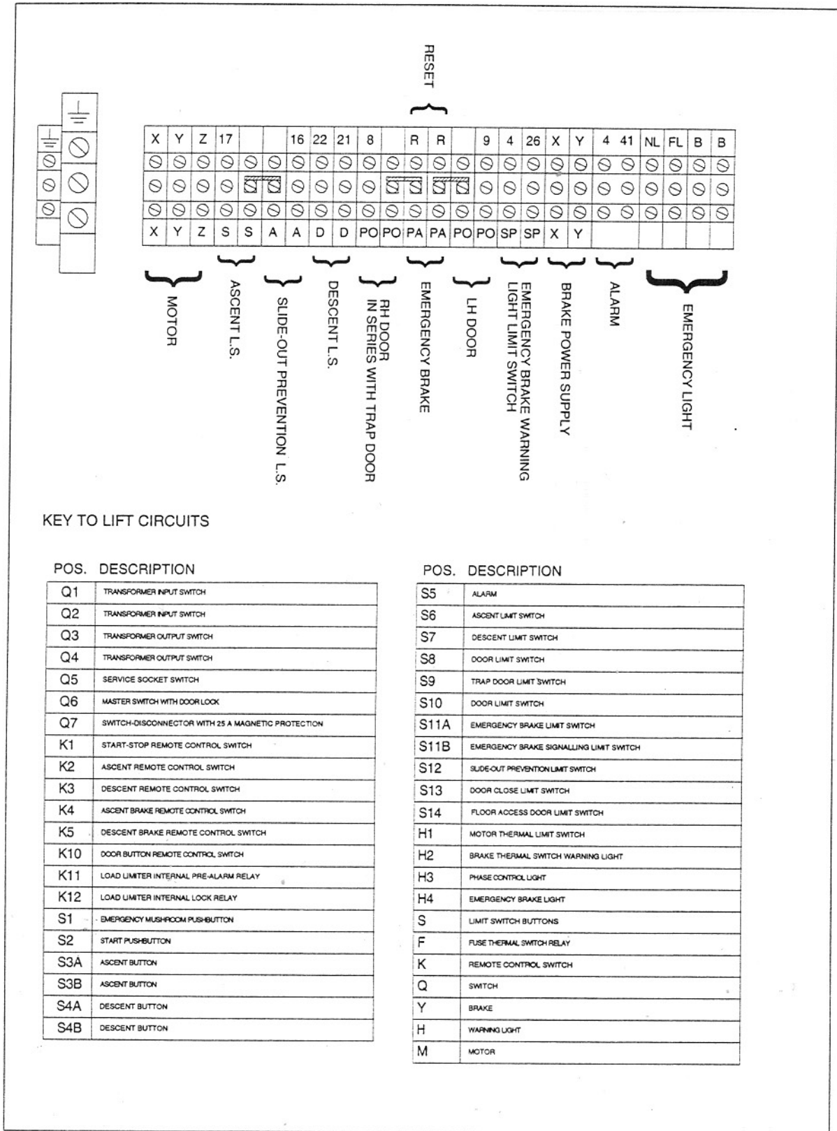
Figure 5.1.3 - Junction terminal board
