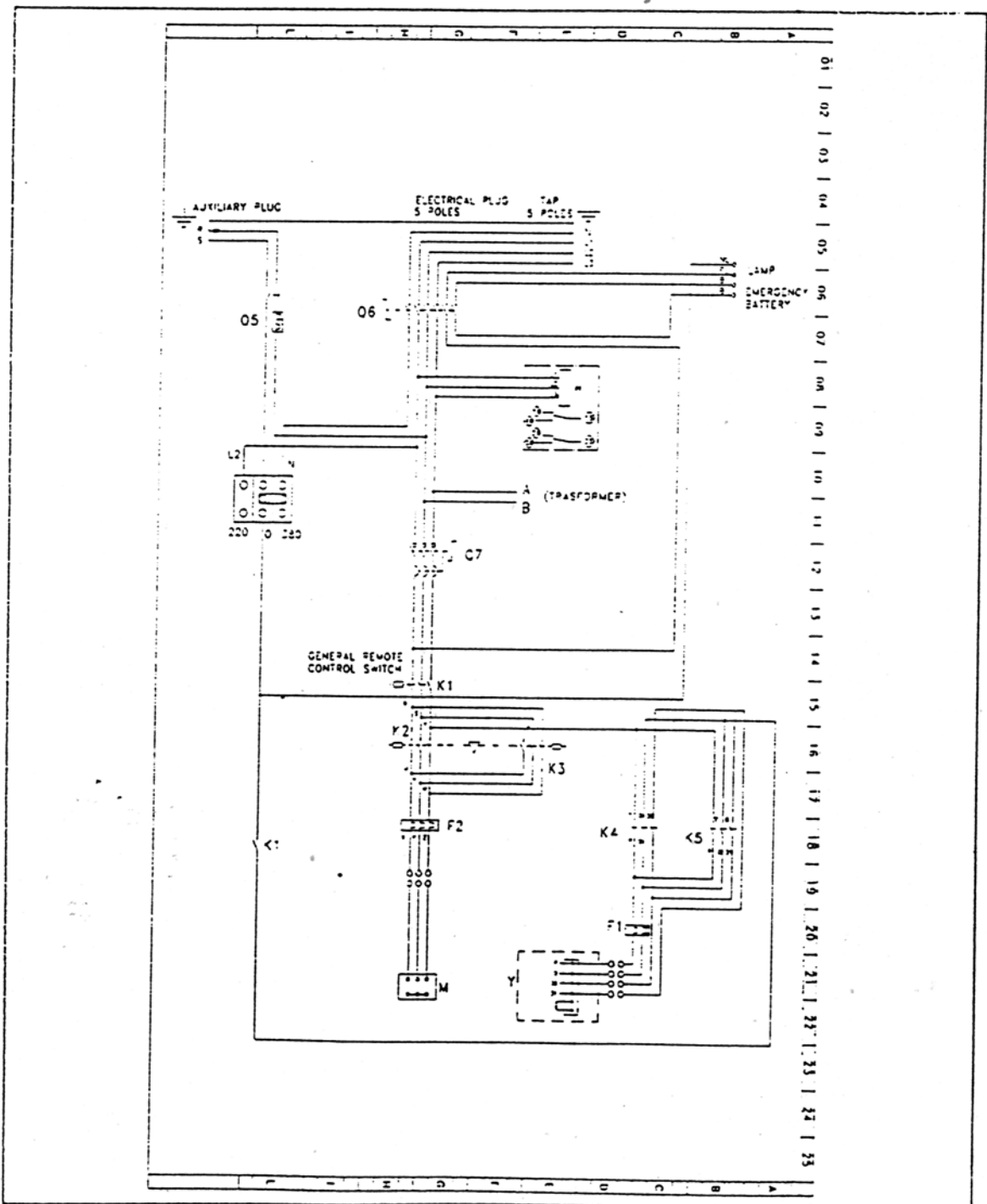
Figure 5.1.1 - Power circuit
