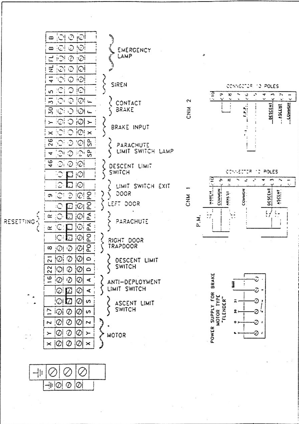
Figure 5.1.3 - Junction terminal board
