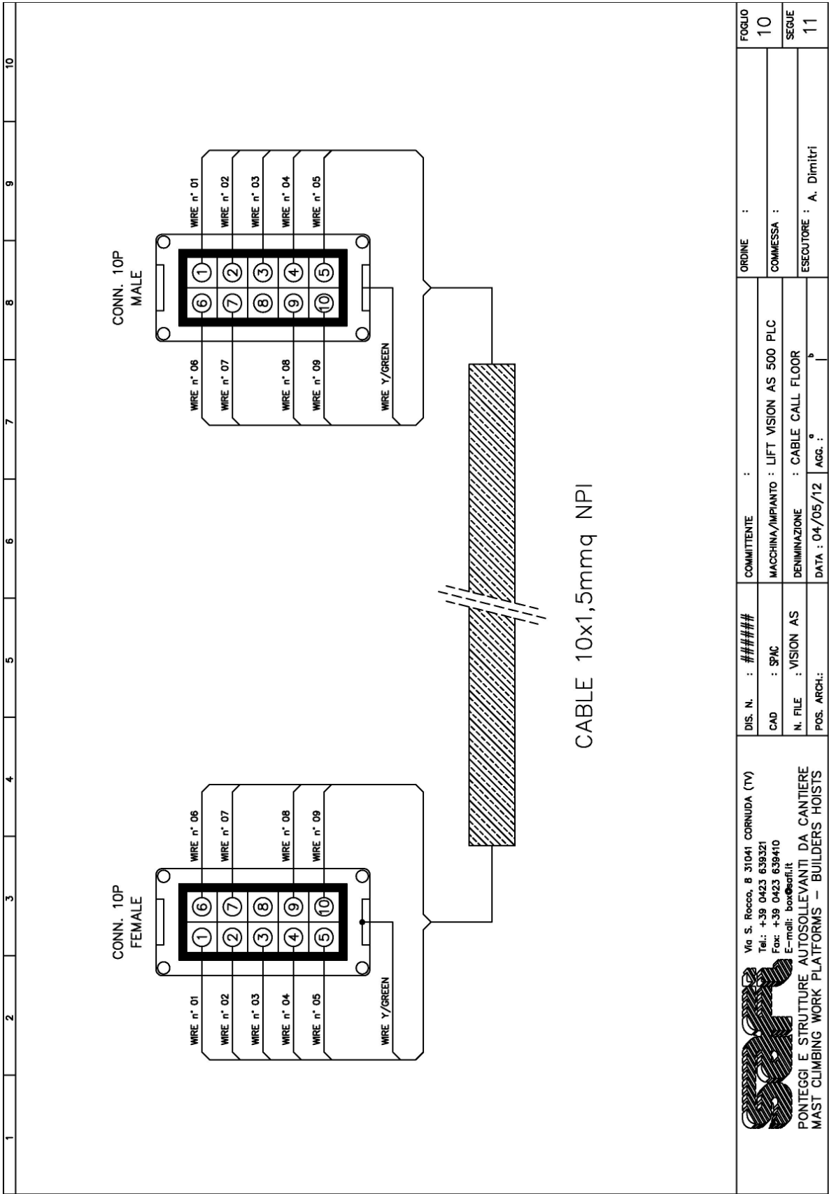
Fig. 12-9 : Wiring diagram – Cable call floor
